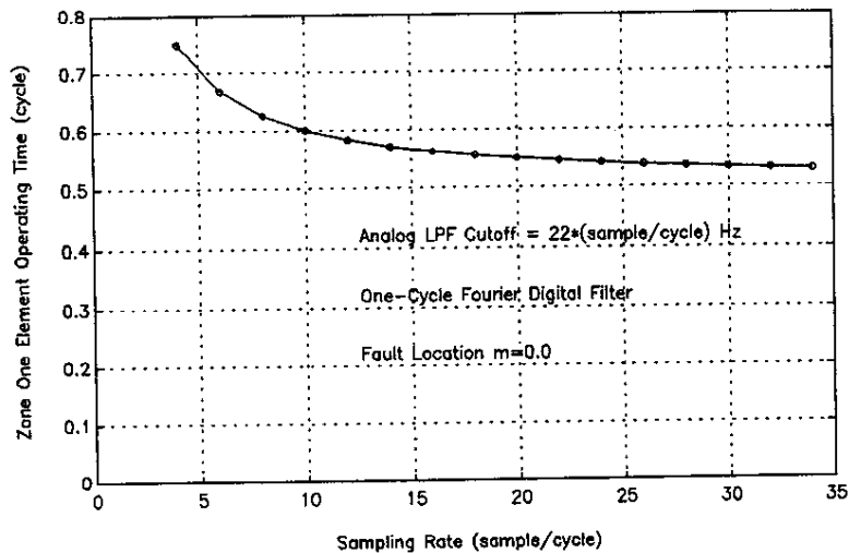
Figure 4.7 Operating Time vs Sampling Rate
