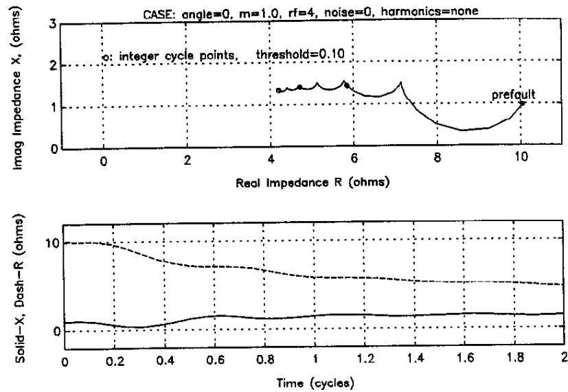
Figure 6.14 Kalman Filter with Threshold 0.10
