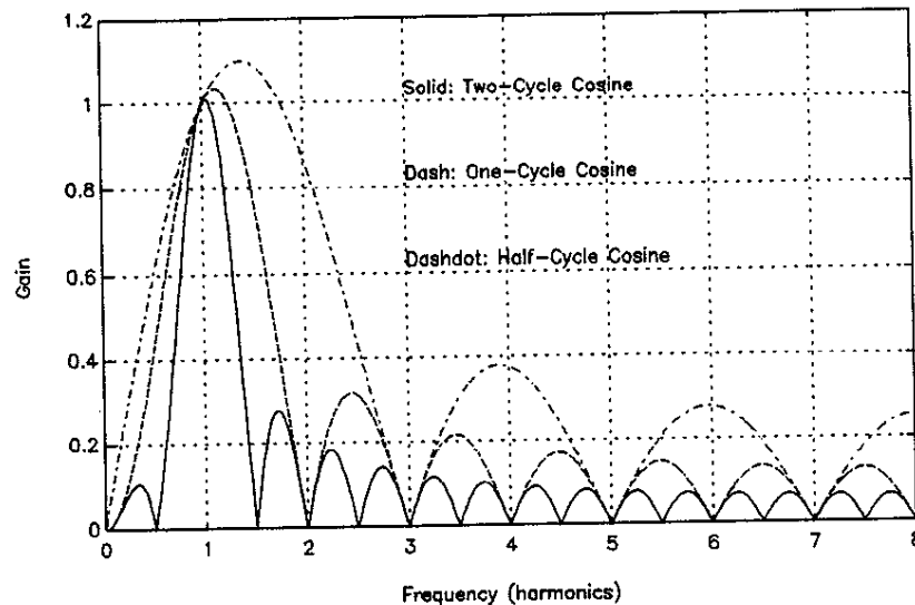
Figure 4.3 Frequency Responses of Half-, One- and Two-Cycle Window Cosine Filters
