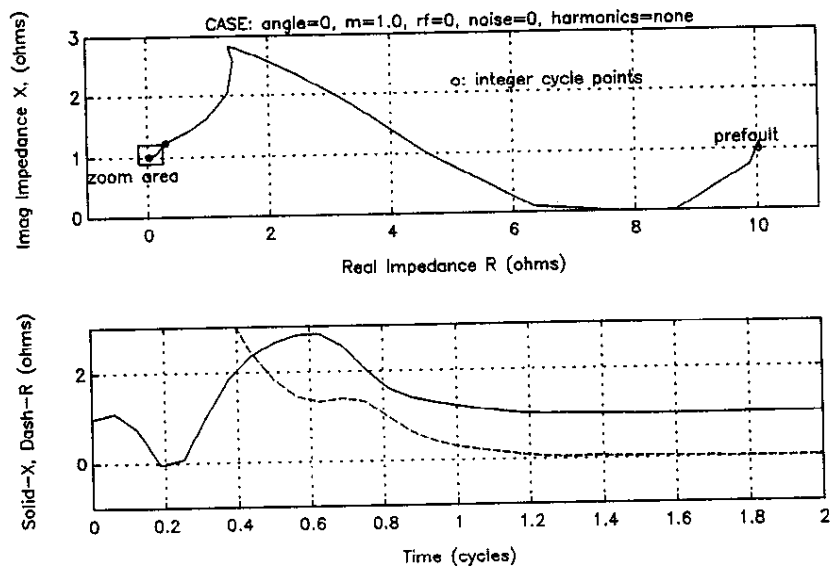
Figure 6.3 Impedance Plot of Cosine Filter
