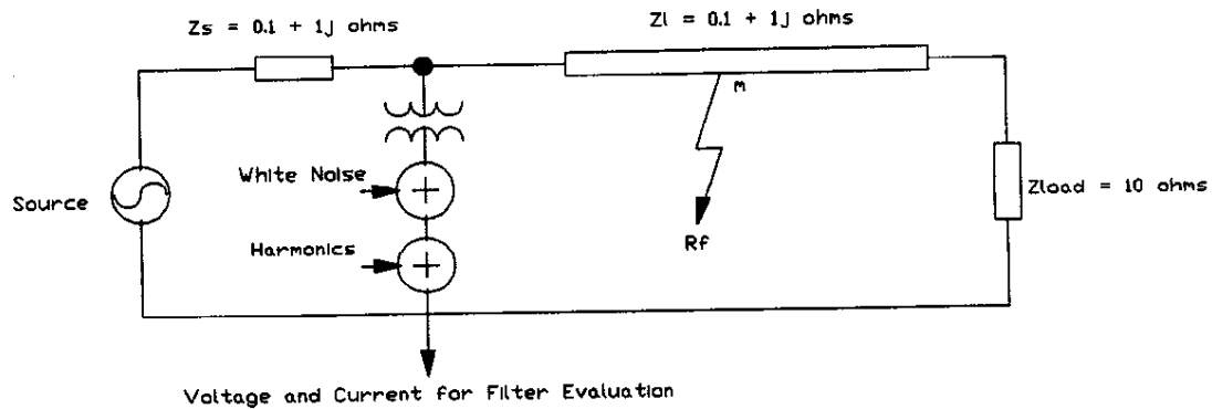
Figure 5.1 Power System Model
