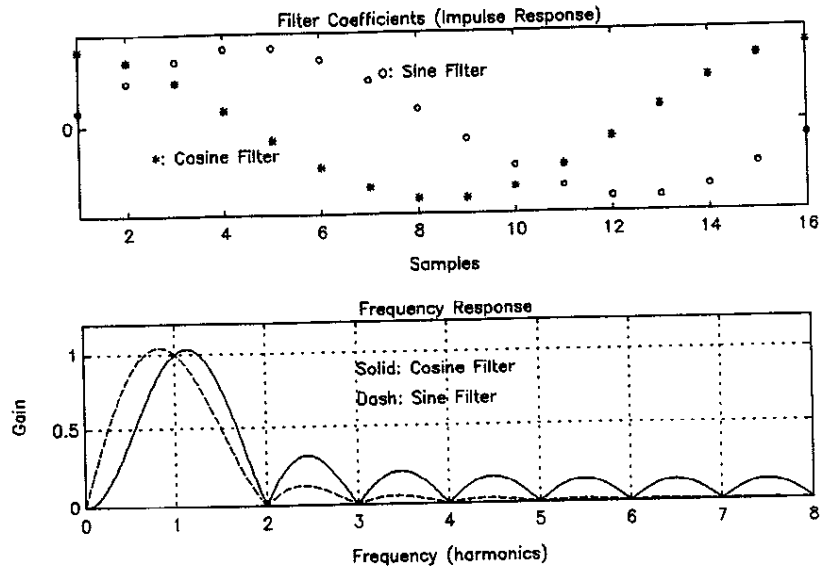
Figure 6.2 Cosine and Sine Filters
