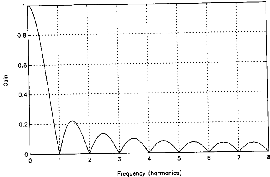
Figure 6.12 FIR LPF of Correlator Filter
