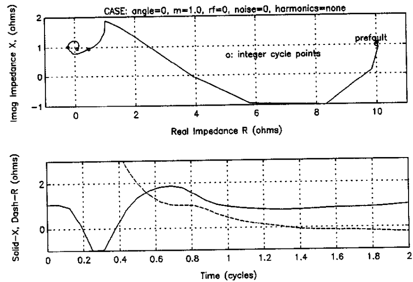
Figure 6.7 Impedance Plot of the IIR Filter
