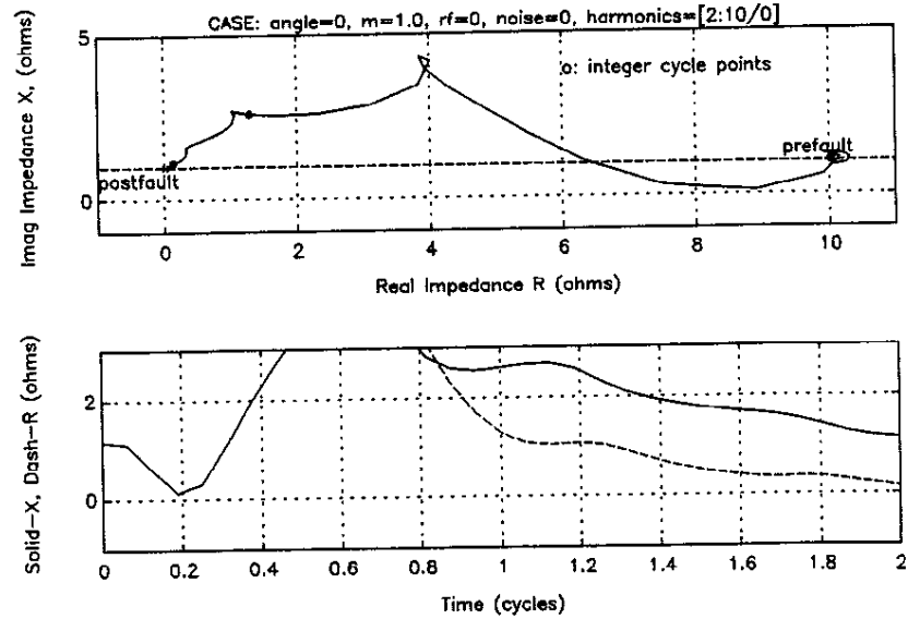
Figure 4.6 Impedance Plot of Two-Cycle Cosine Filter
