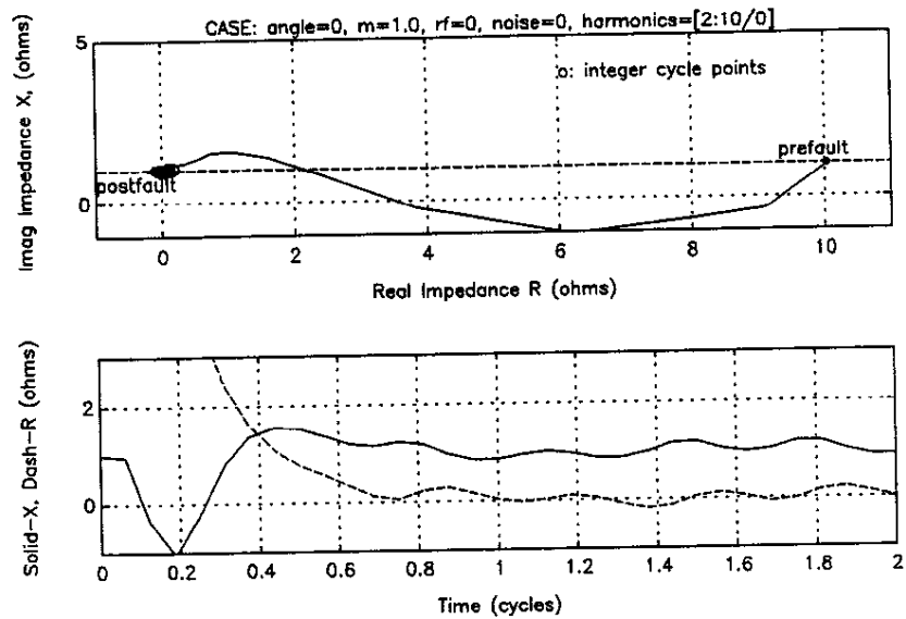
Figure 4.4 Impedance Plot of Half-Cycle Cosine Filter
