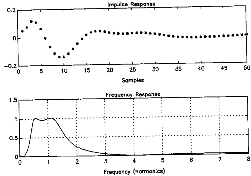
Figure 6.6 An IIR Bandpass Filter
