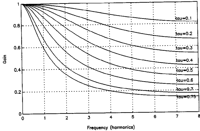
Figure 6.10 IIR LPF of Correlator Filter
