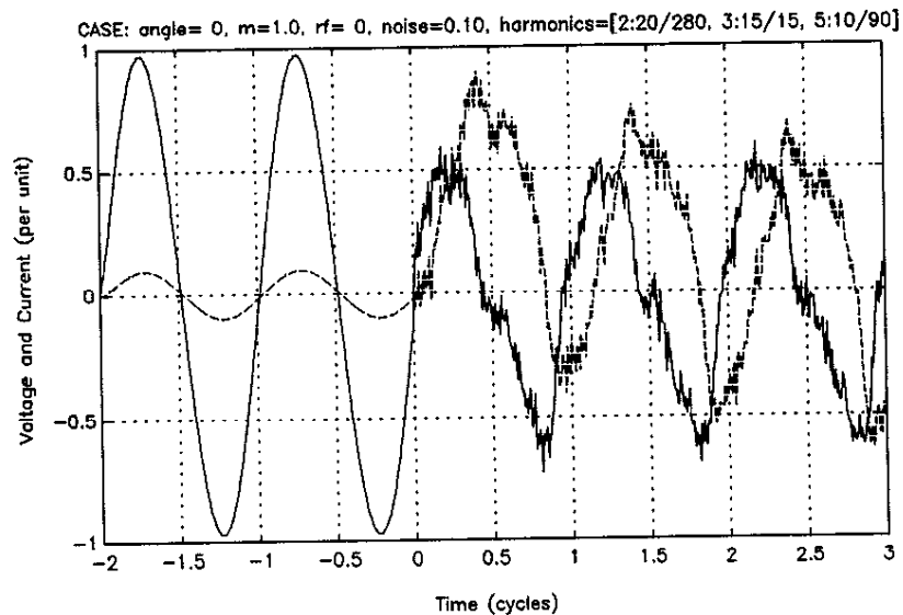
Figure 5.2 Generated Voltage and Current
