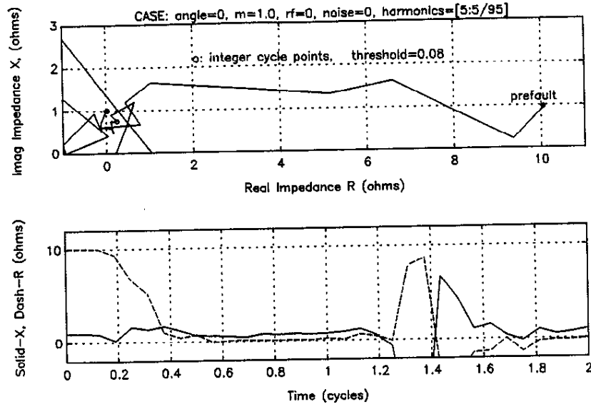
Figure 6.15 Kalman Filter with Threshold 0.08
