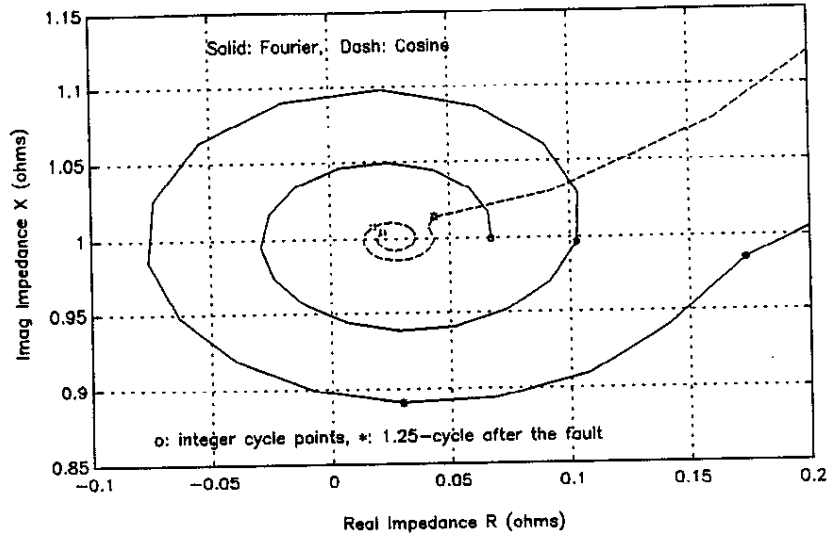
Figure 6.5 Comparison of Cosine and Fourier Filters
