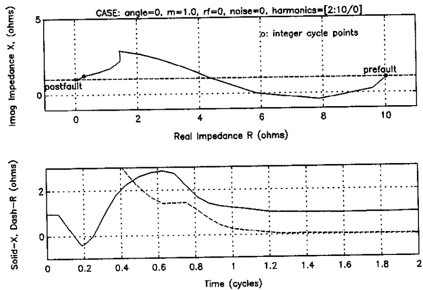
Figure 4.5 Impedance Plot of One-Cycle Cosine Filter
