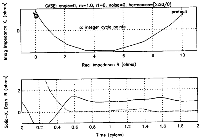
Figure 6.11 Impedance Plot of IIR Correlator Filter
