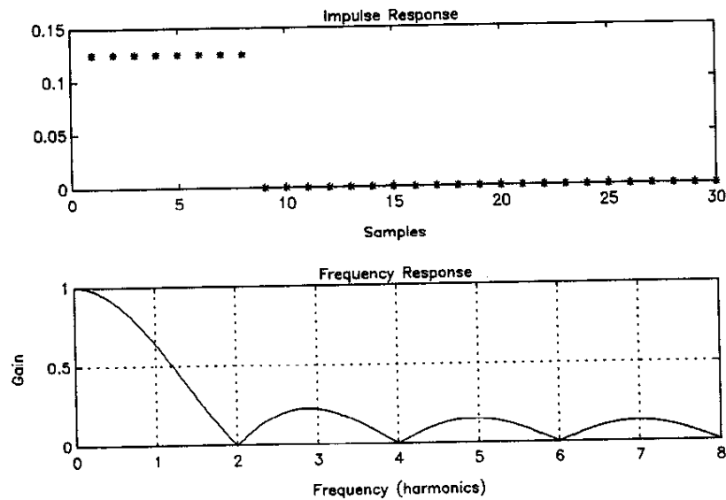
Figure 4.2 FIR Lowpass Filter y_k = [x_k + \dots + x_{k-7}]/8
