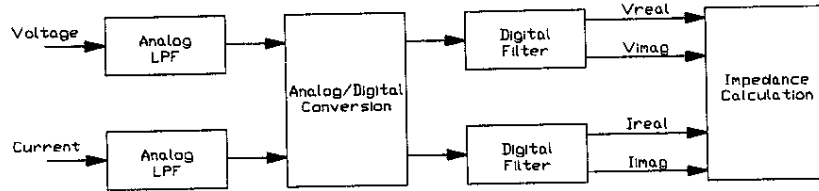
Figure 5.3 System for Evaluating Analog and Digital Filters
