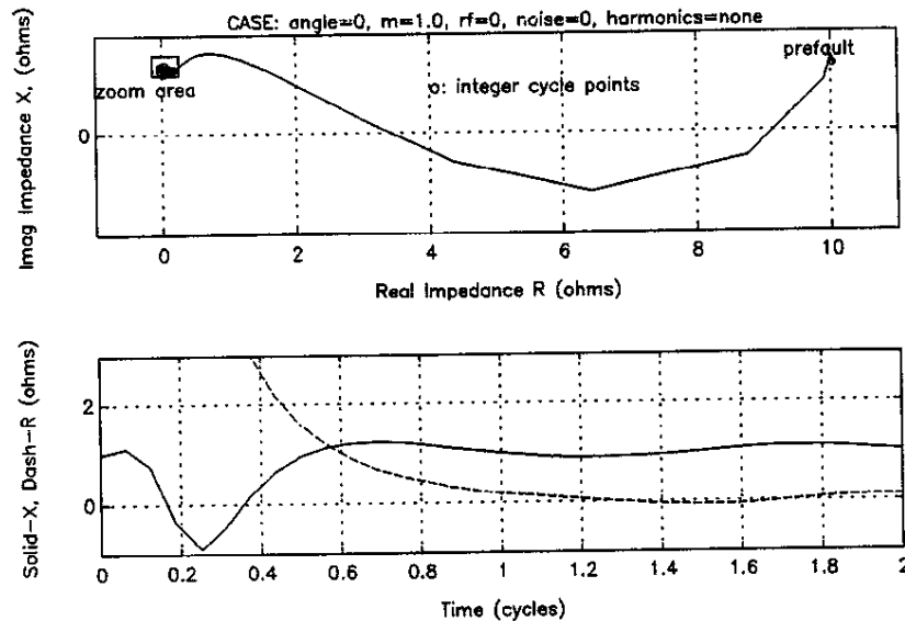
Figure 6.4 Impedance Plot of Fourier Filter
