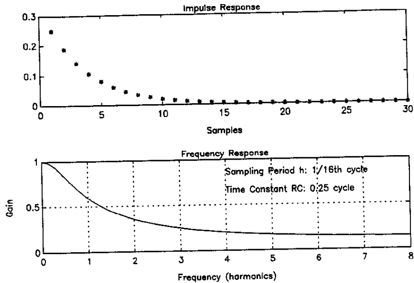
Figure 4.1 IIR Lowpass Filter y_k = (1/4)x_k + [1-(1/4)]y_{k-1}
