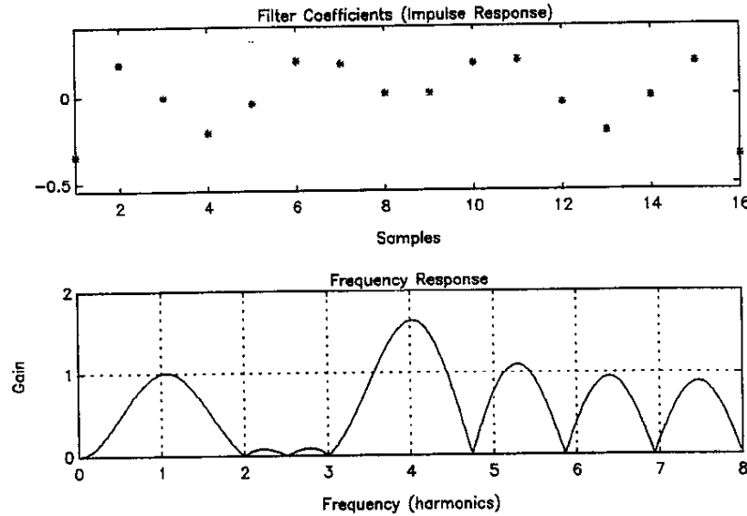
Figure 6.13 One Least-Squares Filter
